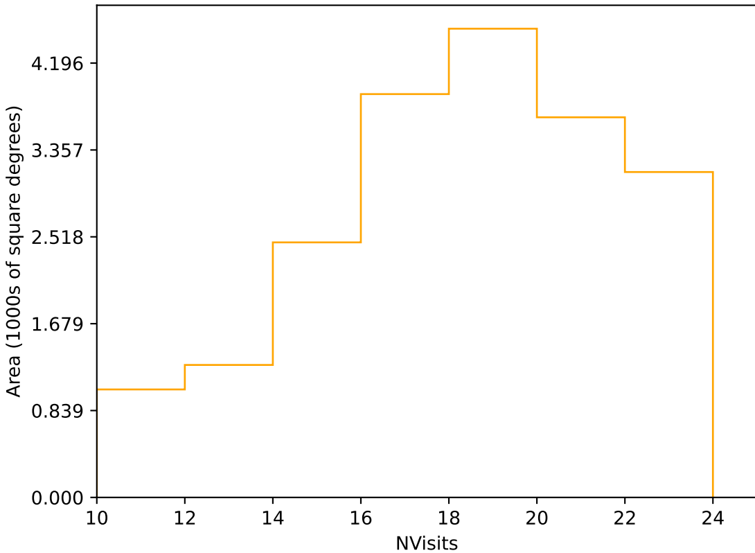
ddf_loaded_half_fl15_v3.4_10yrs Yr 1 r band: NVisits
