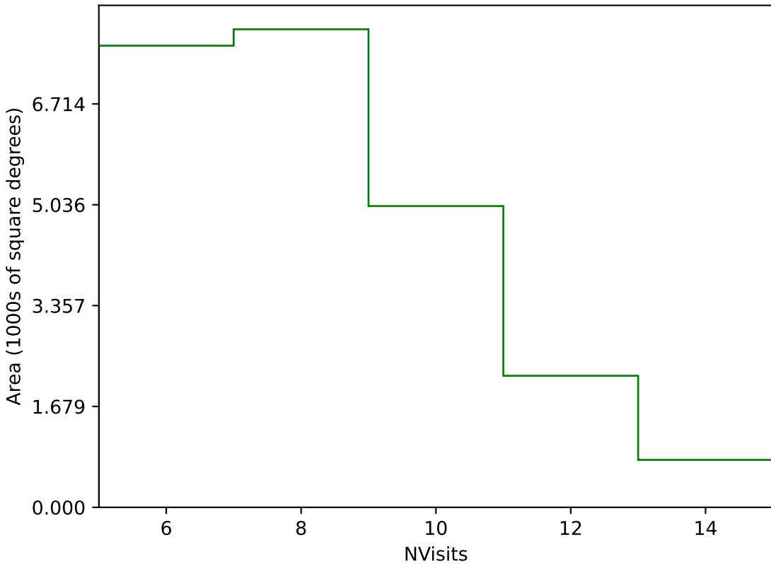
ddf_loaded_half_fl15_v3.4_10yrs Yr 1 g band: NVisits
