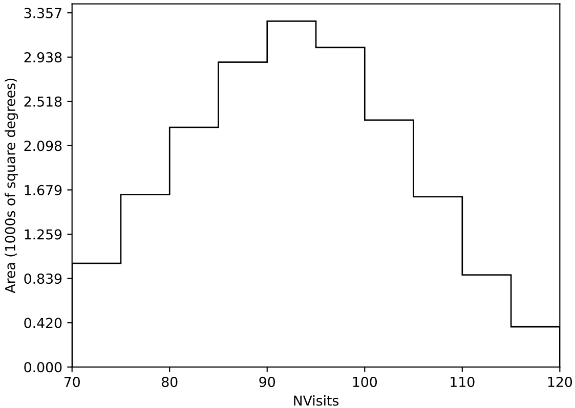
ddf_loaded_half_fl15_v3.4_10yrs Yr 1 all bands: NVisits
