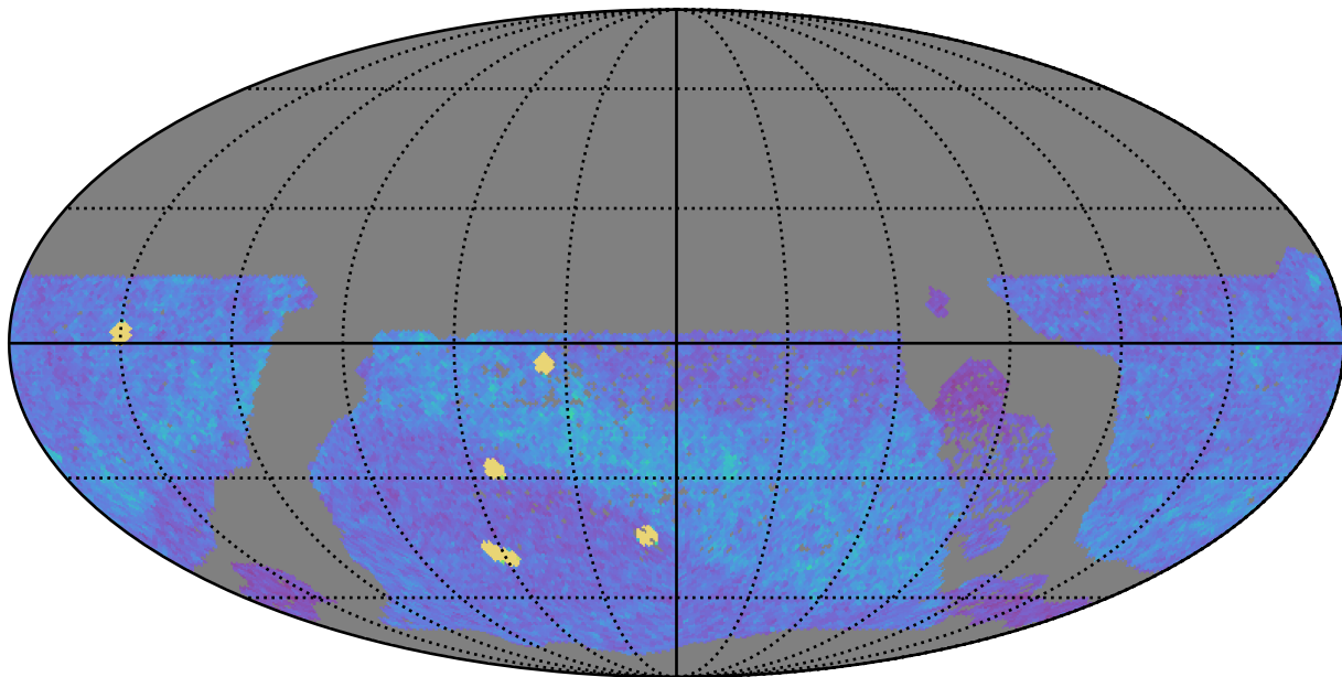
ddf_loaded_half_fl15_v3.4_10yrs WFD z band: NVisits
