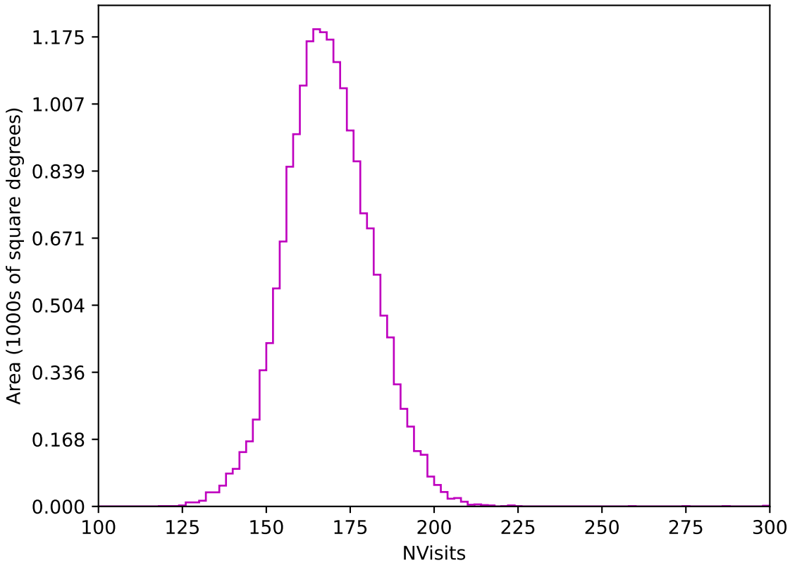
ddf_loaded_half_fl15_v3.4_10yrs WFD z band: NVisits
