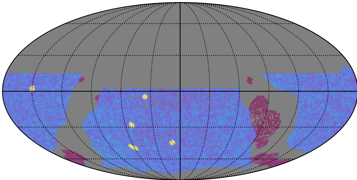
ddf_loaded_half_fl15_v3.4_10yrs WFD y band: NVisits
