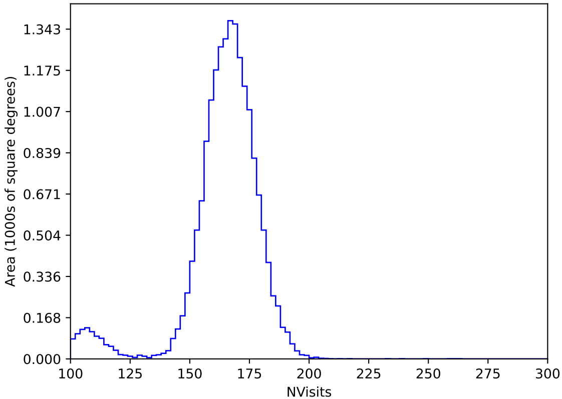
ddf_loaded_half_fl15_v3.4_10yrs WFD y band: NVisits
