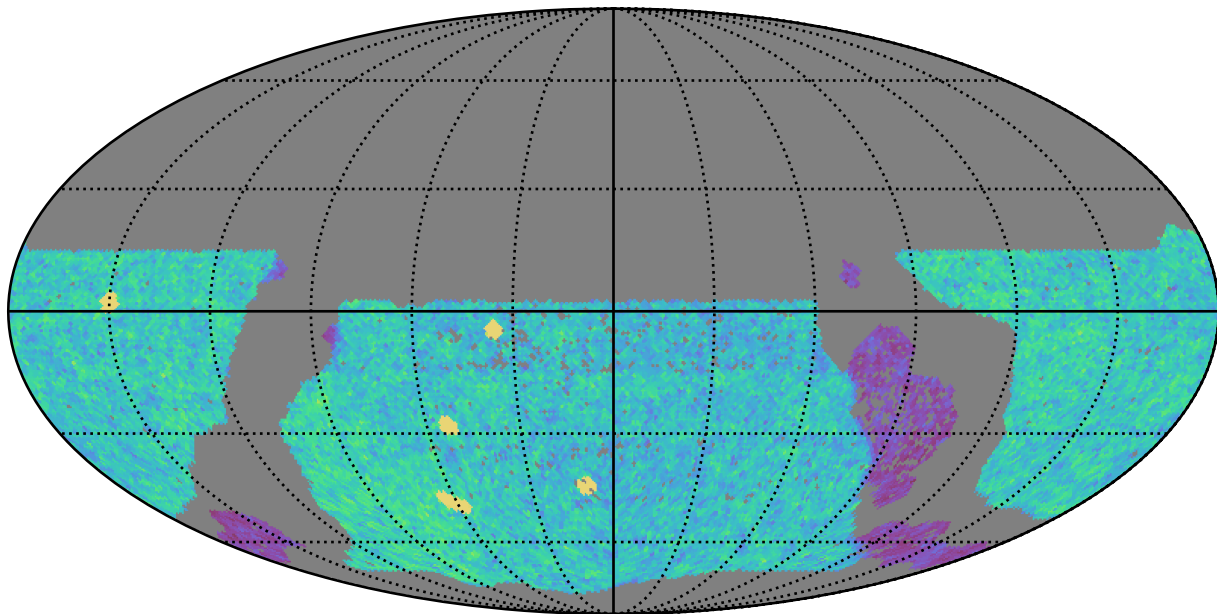
ddf_loaded_half_fl15_v3.4_10yrs WFD u band: NVisits
