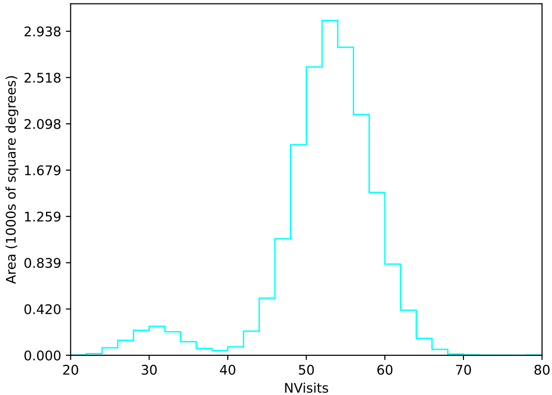
ddf_loaded_half_fl15_v3.4_10yrs WFD u band: NVisits
