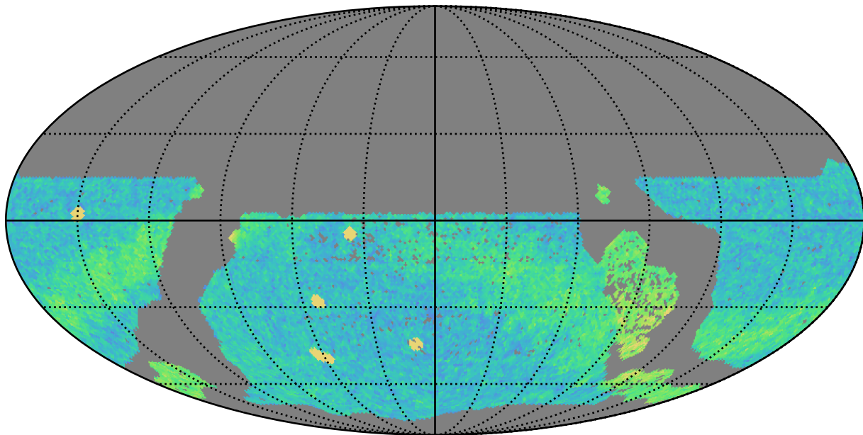
ddf_loaded_half_fl15_v3.4_10yrs WFD r band: NVisits
