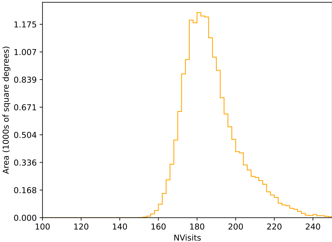
ddf_loaded_half_fl15_v3.4_10yrs WFD r band: NVisits
