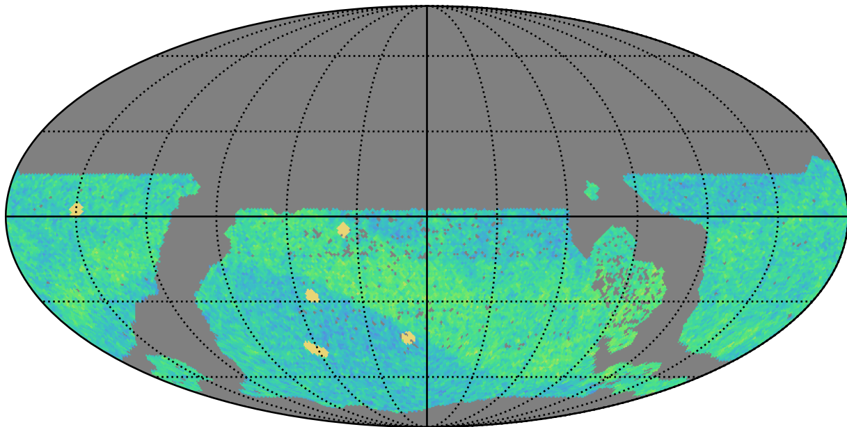
ddf_loaded_half_fl15_v3.4_10yrs WFD i band: NVisits
