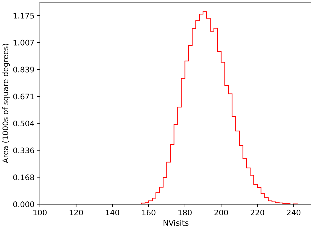
ddf_loaded_half_fl15_v3.4_10yrs WFD i band: NVisits
