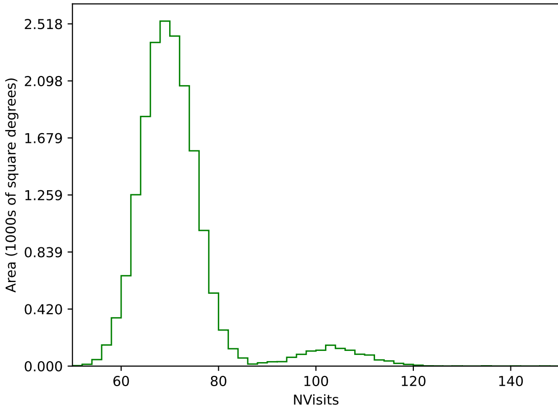
ddf_loaded_half_fl15_v3.4_10yrs WFD g band: NVisits
