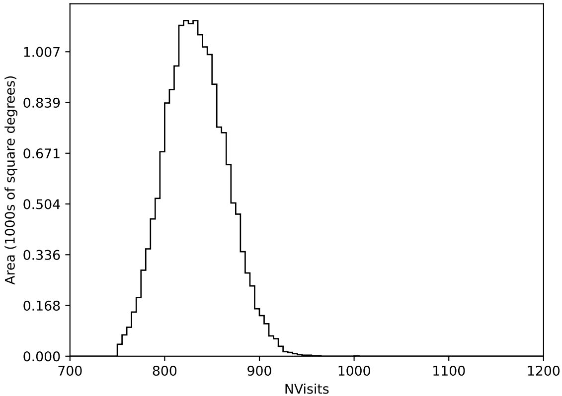
ddf_loaded_half_fl15_v3.4_10yrs WFD all bands: NVisits
