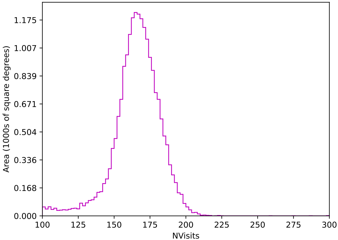
ddf_loaded_half_fl15_v3.4_10yrs All sky z band: NVisits
