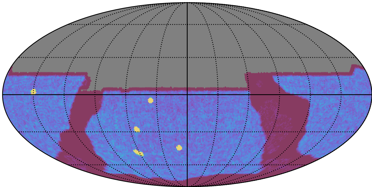
ddf_loaded_half_fl15_v3.4_10yrs All sky y band: NVisits
