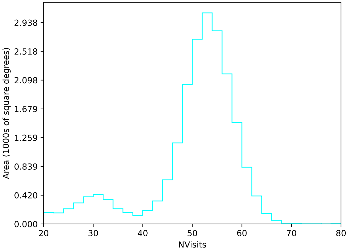
ddf_loaded_half_fl15_v3.4_10yrs All sky u band: NVisits
