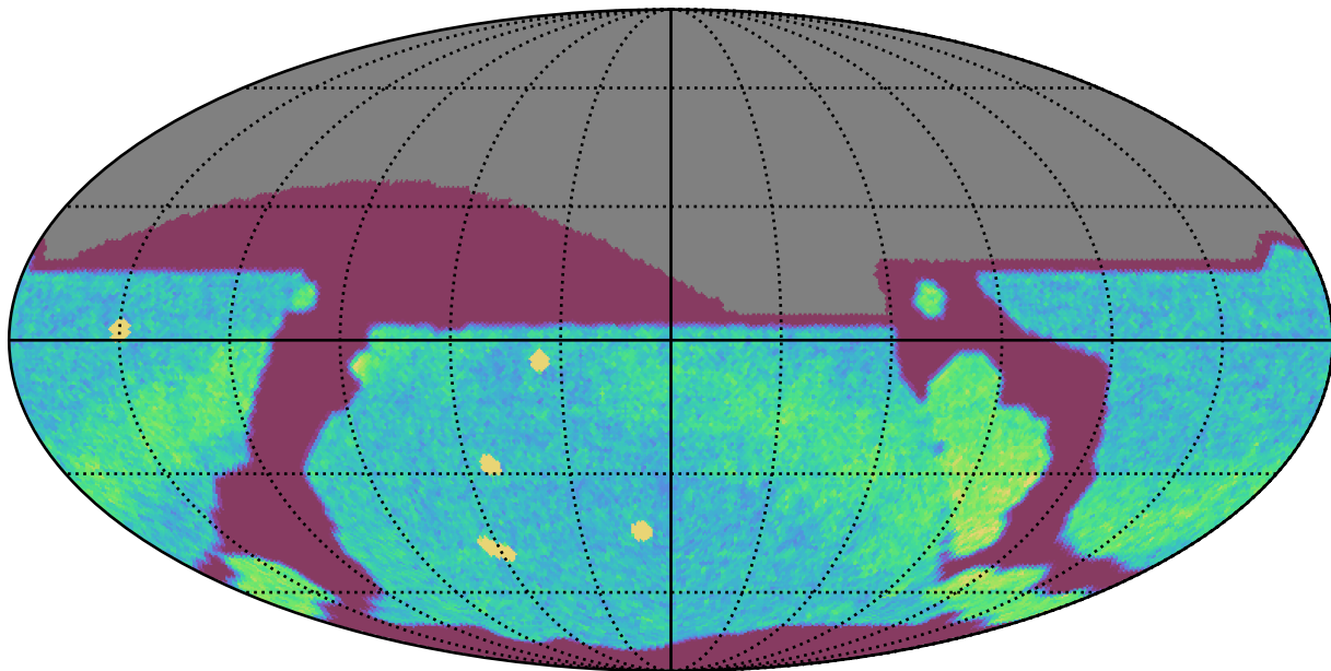
ddf_loaded_half_fl15_v3.4_10yrs All sky r band: NVisits
