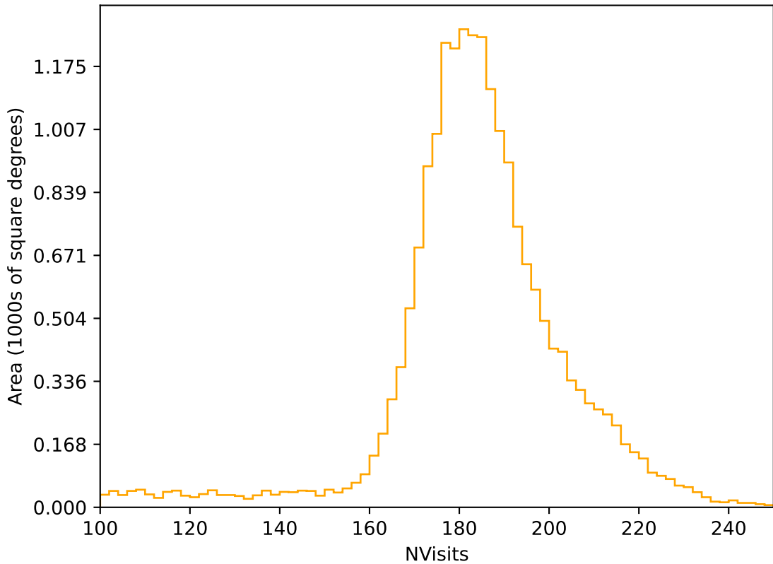
ddf_loaded_half_fl15_v3.4_10yrs All sky r band: NVisits
