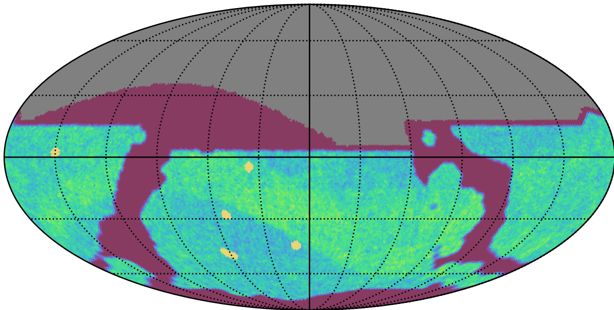
ddf_loaded_half_fl15_v3.4_10yrs All sky i band: NVisits
