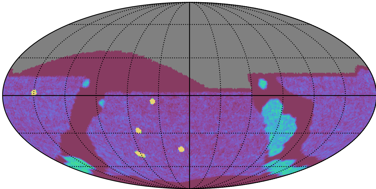
ddf_loaded_half_fl15_v3.4_10yrs All sky g band: NVisits
