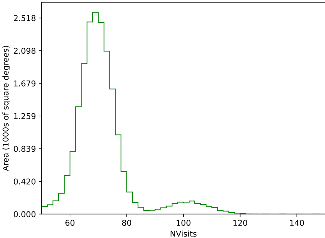
ddf_loaded_half_fl15_v3.4_10yrs All sky g band: NVisits
