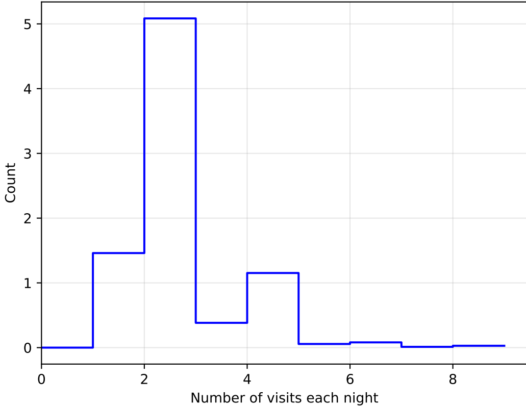
ddf_loaded_half_fl15_v3.4_10yrs WFD: NVisitsPerNight
