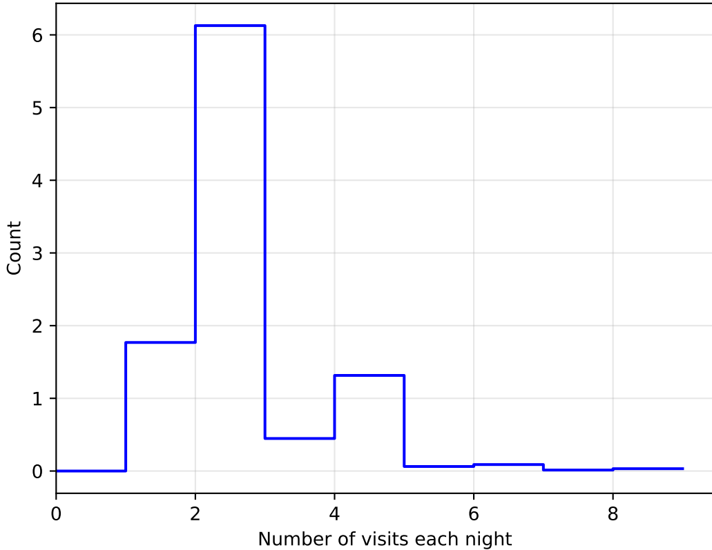
ddf_loaded_half_fl15_v3.4_10yrs All sky: NVisitsPerNight
