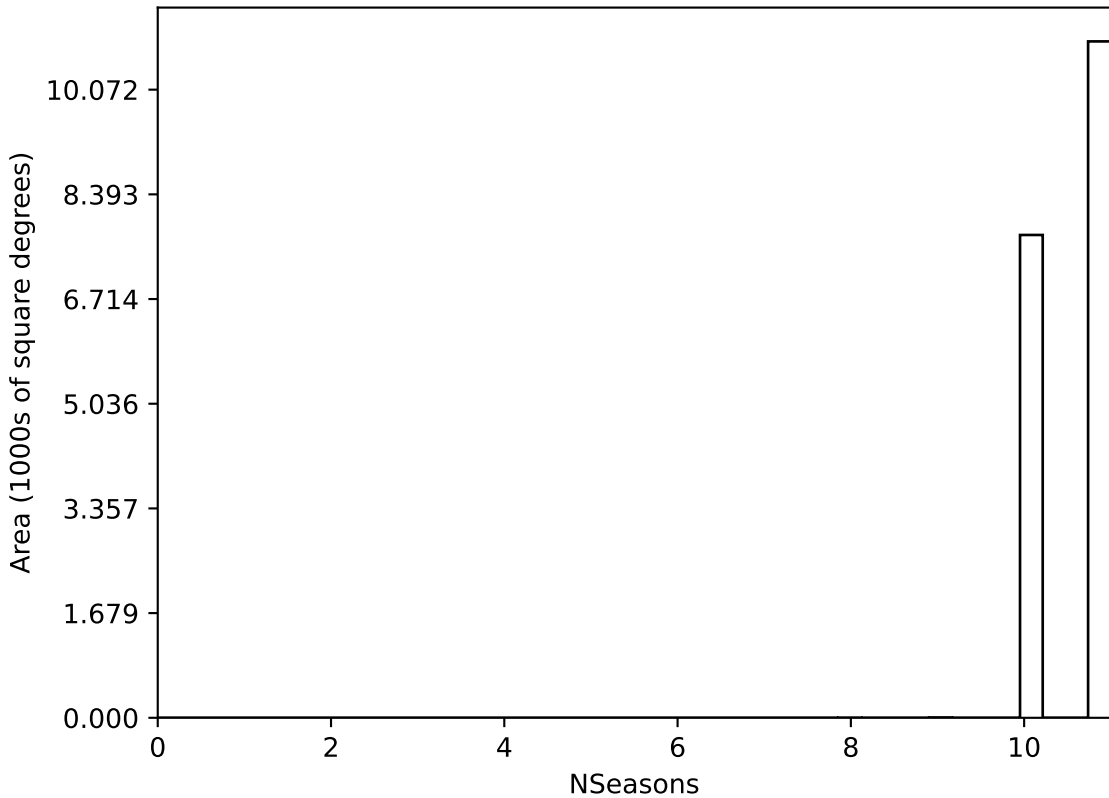
ddf_loaded_half_fl15_v3.4_10yrs WFD all bands: NSeasons
