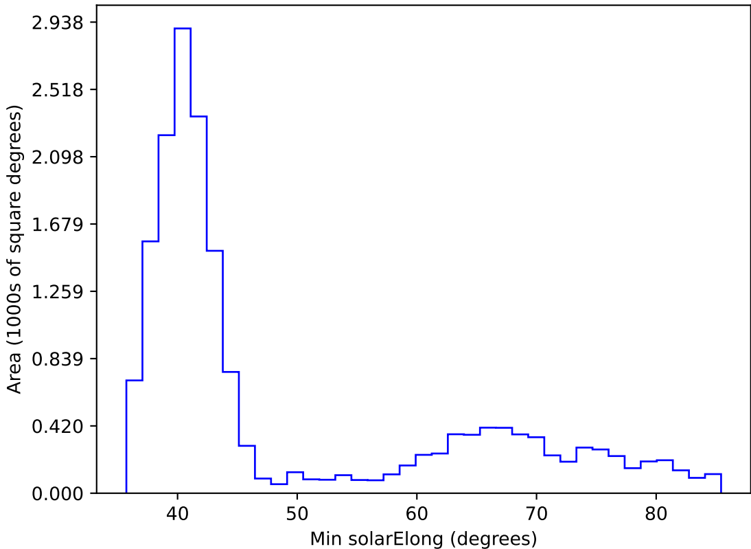
ddf_loaded_half_fl15_v3.4_10yrs WFD z band: Min solarElong
