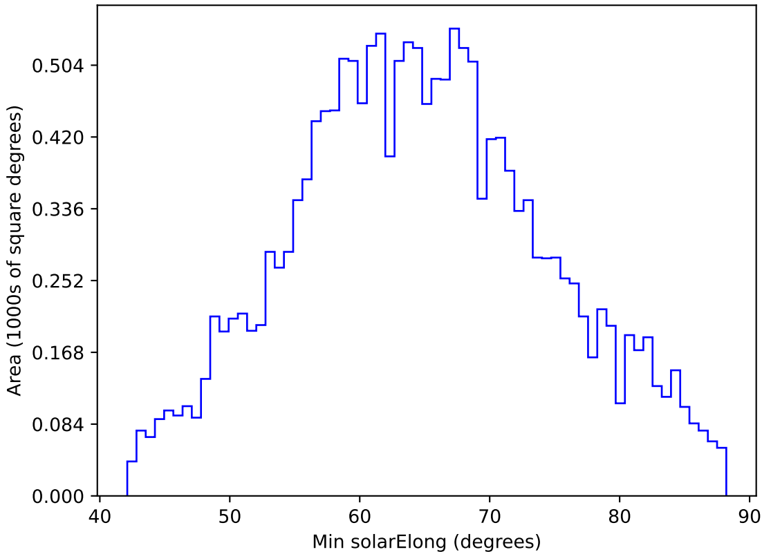
ddf_loaded_half_fl15_v3.4_10yrs WFD y band: Min solarElong
