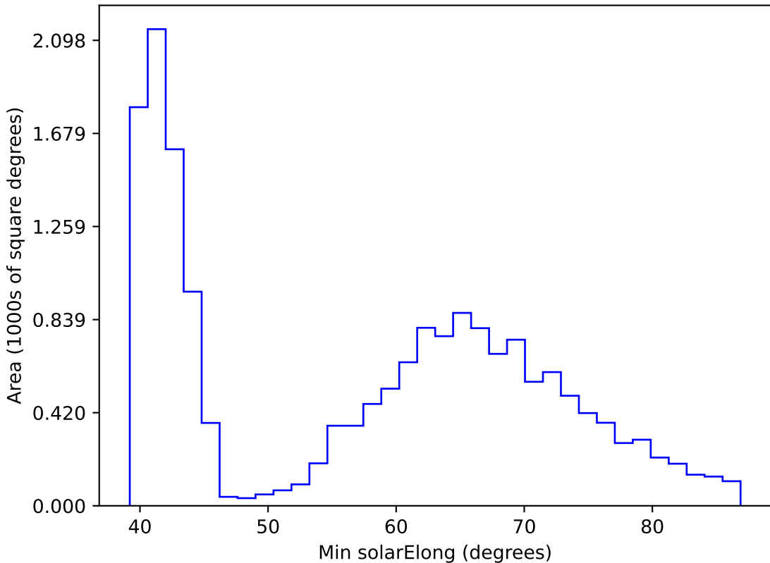
ddf_loaded_half_fl15_v3.4_10yrs WFD r band: Min solarElong
