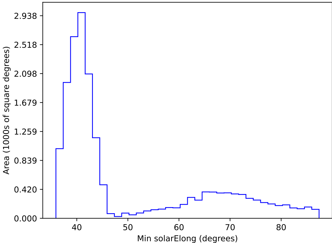
ddf_loaded_half_fl15_v3.4_10yrs WFD i band: Min solarElong
