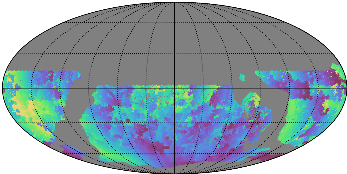
ddf_loaded_half_fl15_v3.4_10yrs WFD g band: Min solarElong
