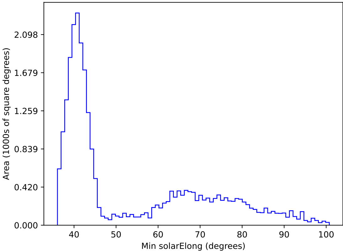
ddf_loaded_half_fl15_v3.4_10yrs All sky z band: Min solarElong
