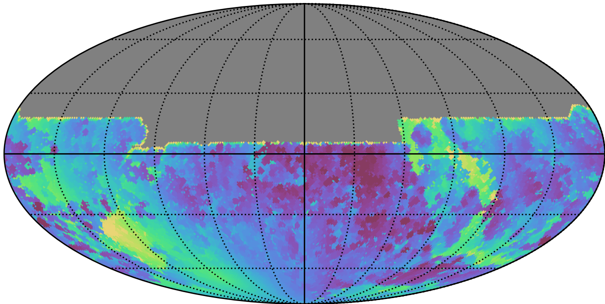
ddf_loaded_half_fl15_v3.4_10yrs All sky y band: Min solarElong
