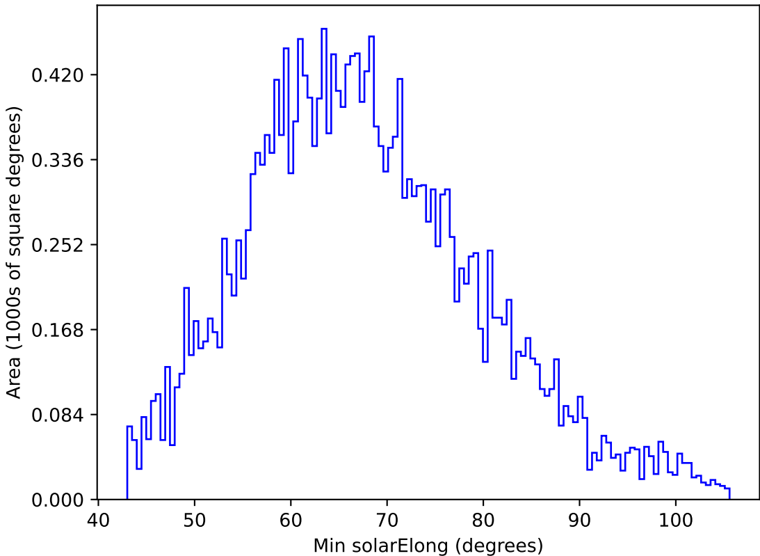
ddf_loaded_half_fl15_v3.4_10yrs All sky y band: Min solarElong
