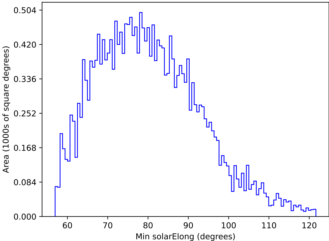
ddf_loaded_half_fl15_v3.4_10yrs All sky u band: Min solarElong
