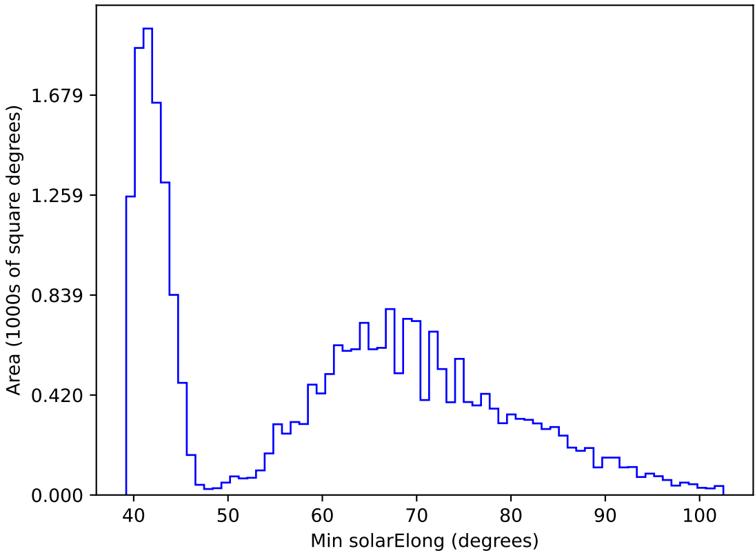
ddf_loaded_half_fl15_v3.4_10yrs All sky r band: Min solarElong
