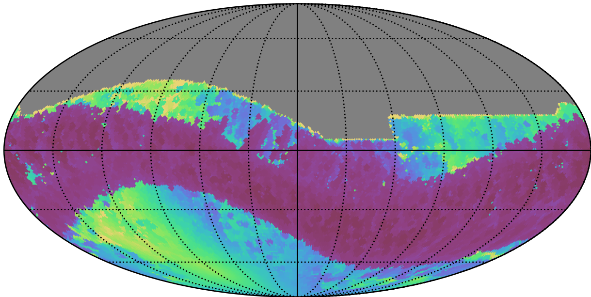
ddf_loaded_half_fl15_v3.4_10yrs All sky i band: Min solarElong
