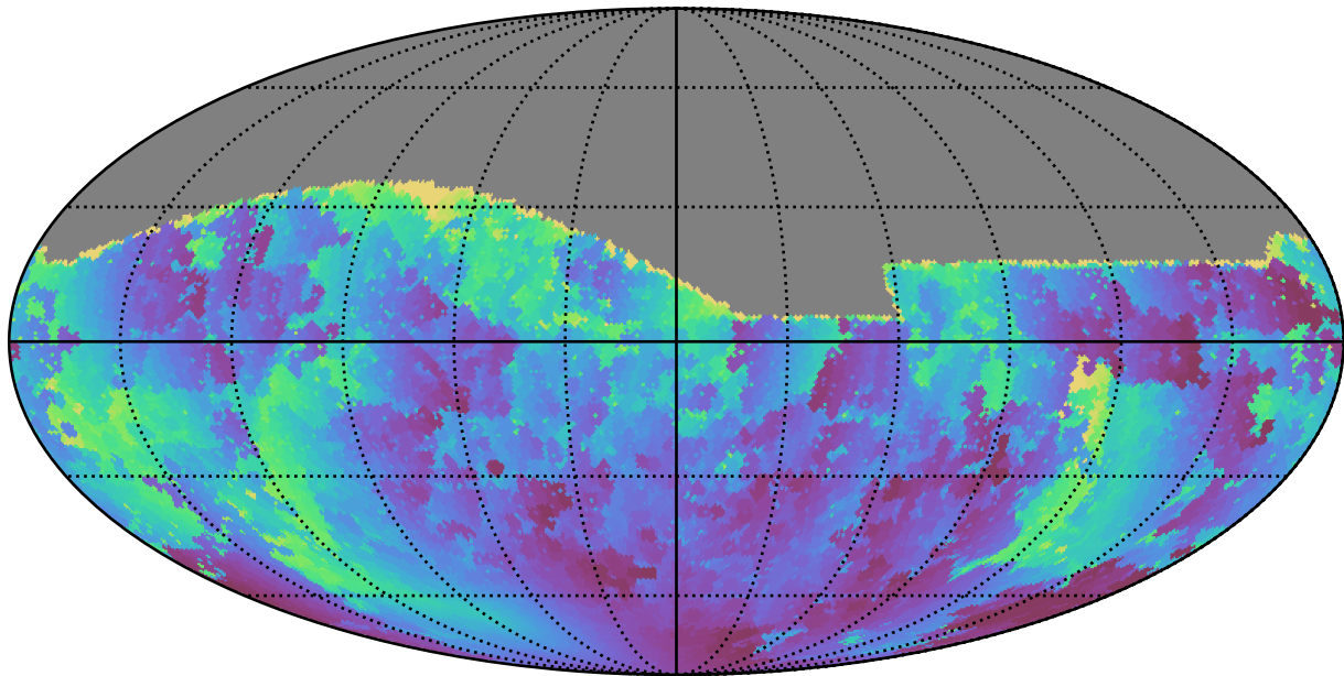
ddf_loaded_half_fl15_v3.4_10yrs All sky g band: Min solarElong
