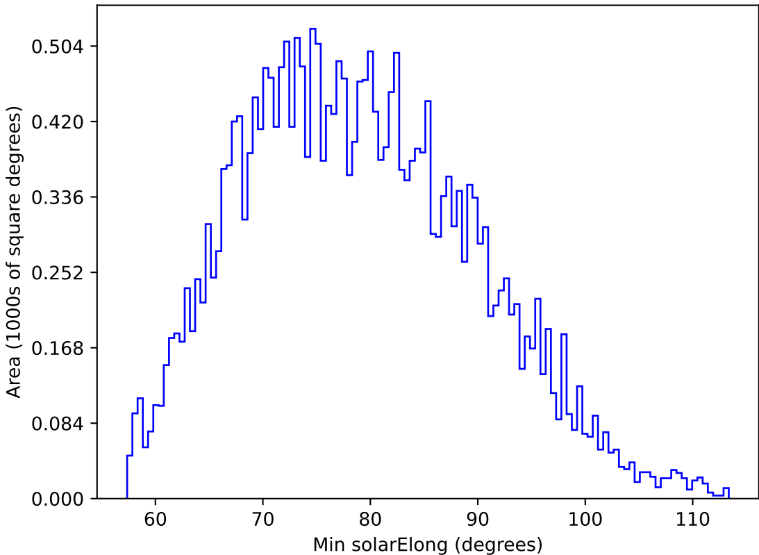
ddf_loaded_half_fl15_v3.4_10yrs All sky g band: Min solarElong
