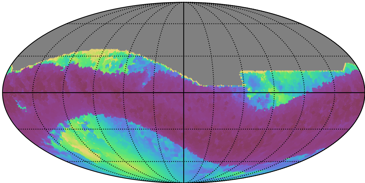
ddf_loaded_half_fl15_v3.4_10yrs All sky all bands: Min solarElong
