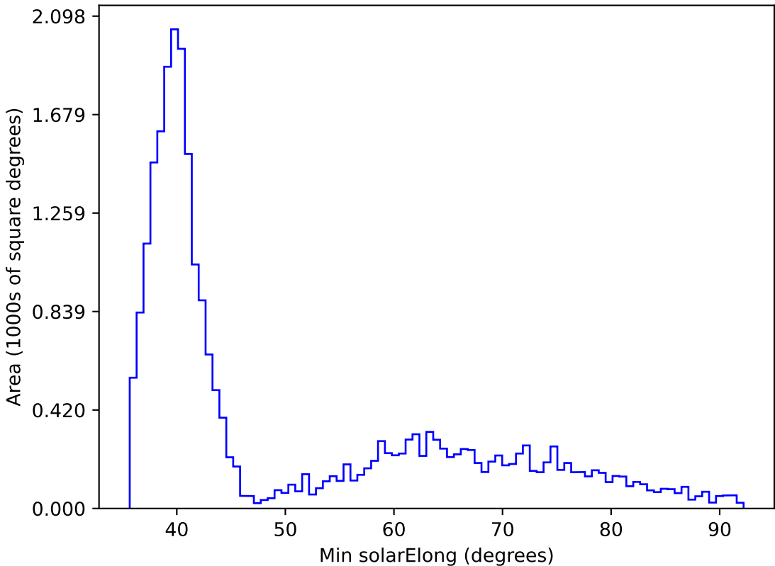
ddf_loaded_half_fl15_v3.4_10yrs All sky all bands: Min solarElong
