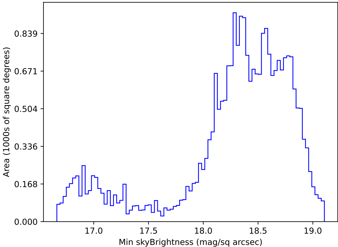
ddf_loaded_half_fl15_v3.4_10yrs Yr 1 z band: Min skyBrightness
