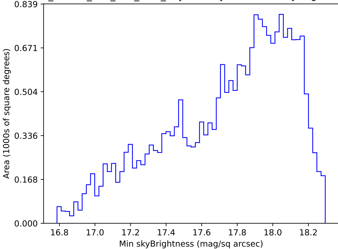
ddf_loaded_half_fl15_v3.4_10yrs Yr 1 y band: Min skyBrightness
