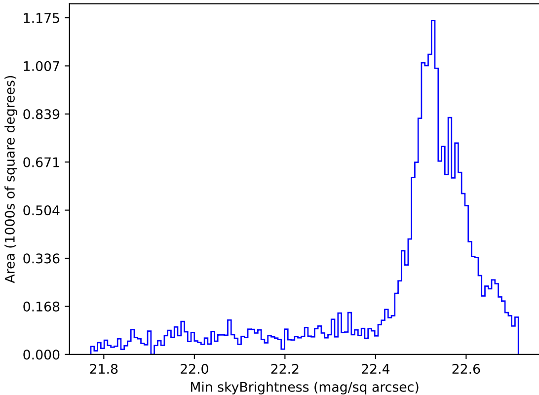
ddf_loaded_half_fl15_v3.4_10yrs Yr 1 u band: Min skyBrightness
