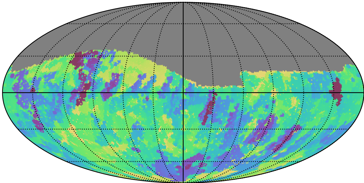
ddf_loaded_half_fl15_v3.4_10yrs Yr 1 r band: Min skyBrightness
