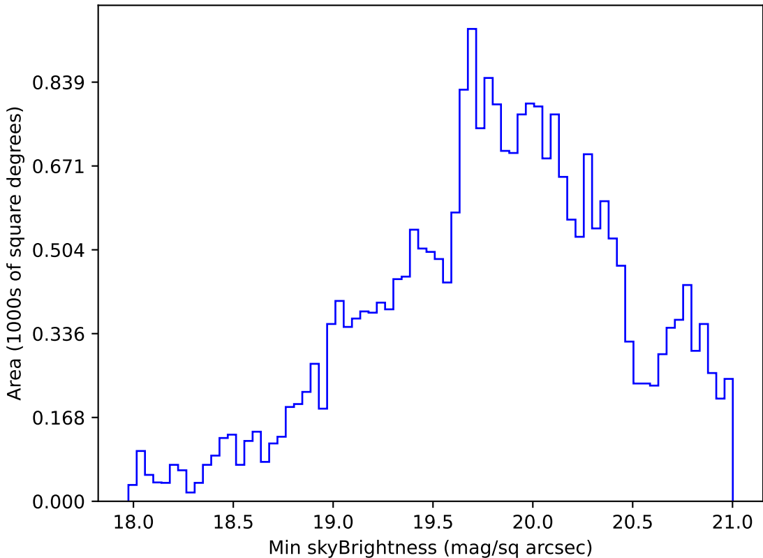
ddf_loaded_half_fl15_v3.4_10yrs Yr 1 r band: Min skyBrightness
