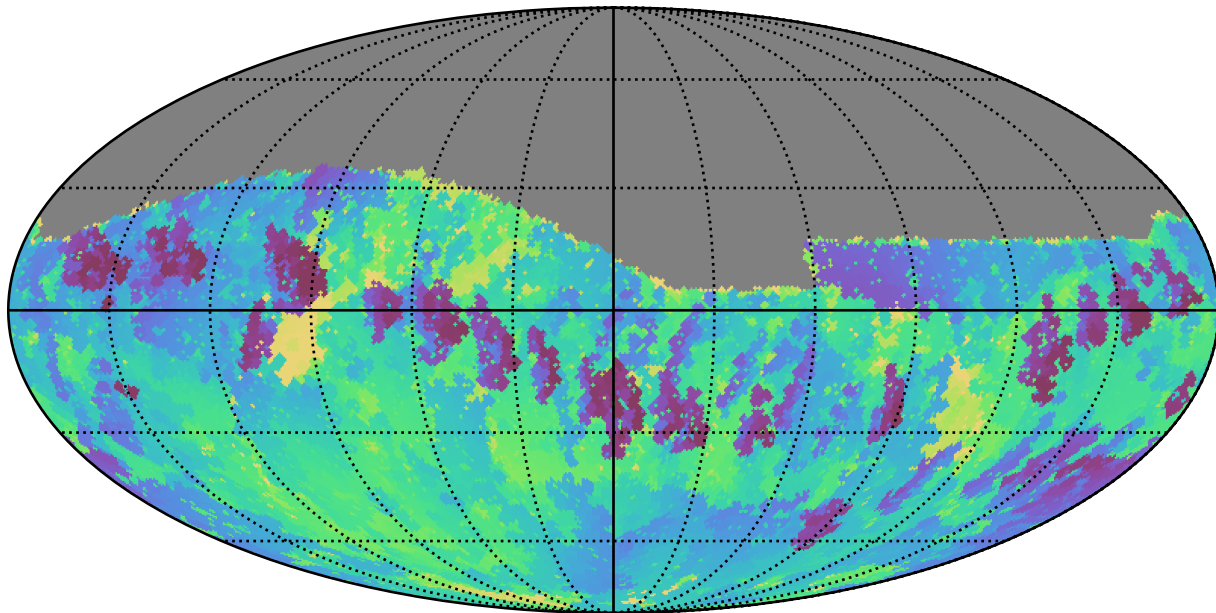
ddf_loaded_half_fl15_v3.4_10yrs Yr 1 i band: Min skyBrightness
