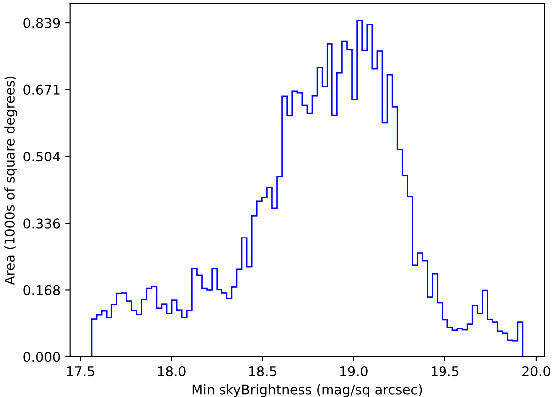
ddf_loaded_half_fl15_v3.4_10yrs Yr 1 i band: Min skyBrightness
