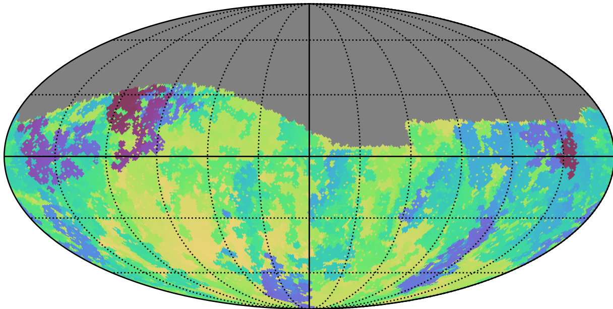
ddf_loaded_half_fl15_v3.4_10yrs Yr 1 g band: Min skyBrightness
