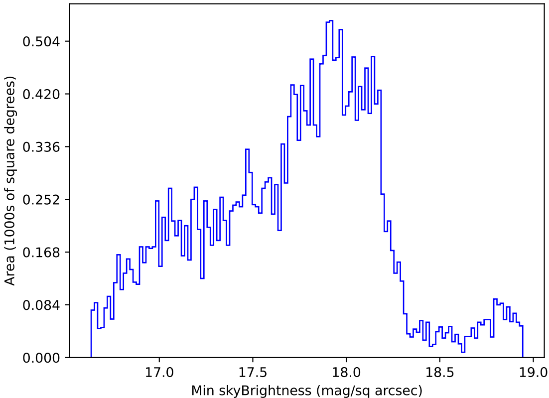
ddf_loaded_half_fl15_v3.4_10yrs Yr 1 all bands: Min skyBrightness
